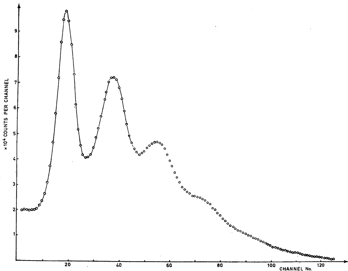
Figure IV-3 - Measured pulse-height distribution of ^{55}\text{Fe} (73 Hou) (courtesy North-Holland Publishing Company, Amsterdam).
