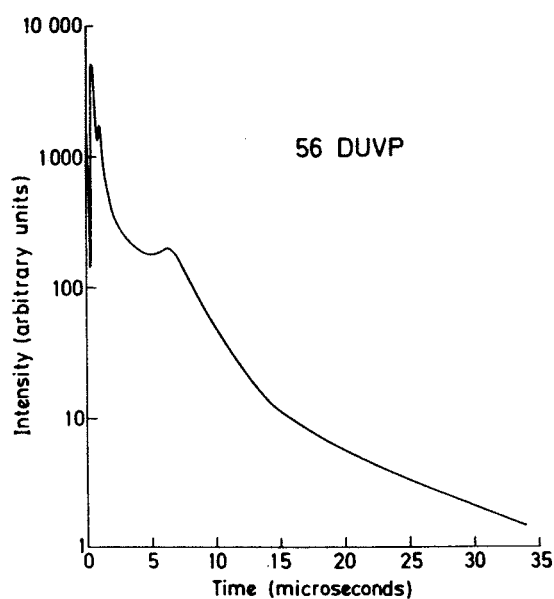
Figure VI-1 - Typical time distribution of afterpulses from 56 DUVP tube.
