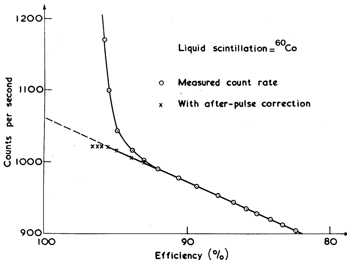
Figure VI-4 - Observed \beta -count rate as a function of measured \beta -counting efficiency, with and without the correction for afterpulsing.
