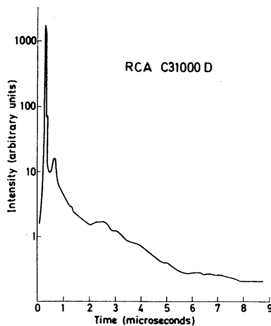
Figure VI-2 - Typical time distribution of afterpulses from RCA 31000D tube.
