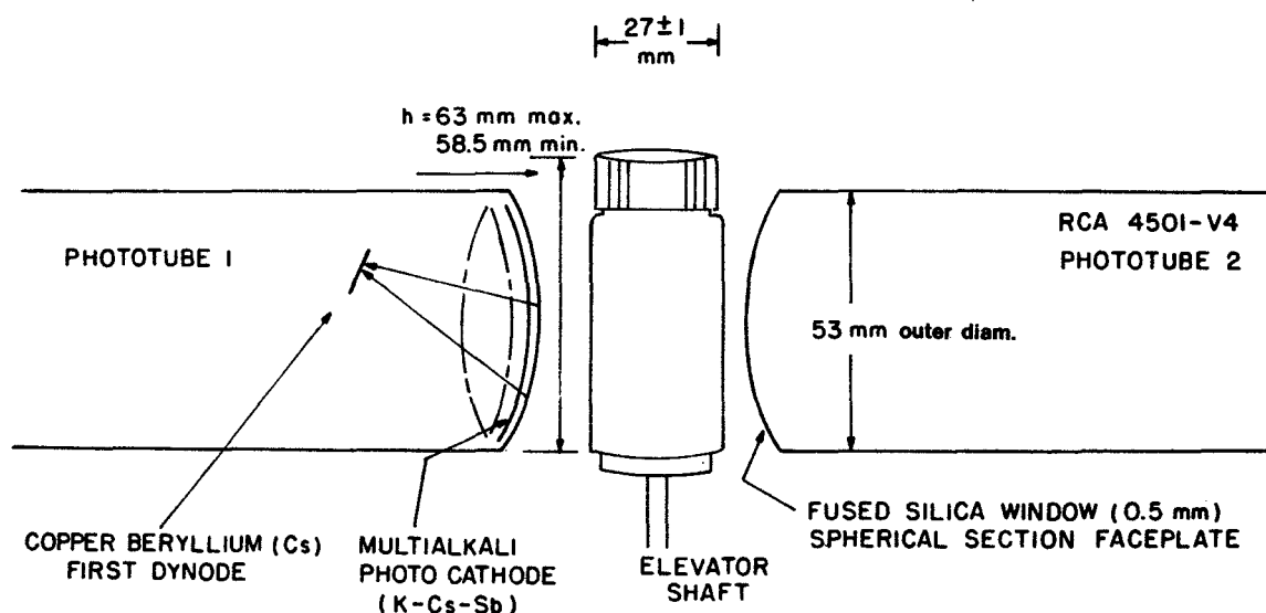
Figure III-1 - Schematic diagram of standard counting vial and phototubes used for typical commercial LS counter (Packard TriCarb 3320).
