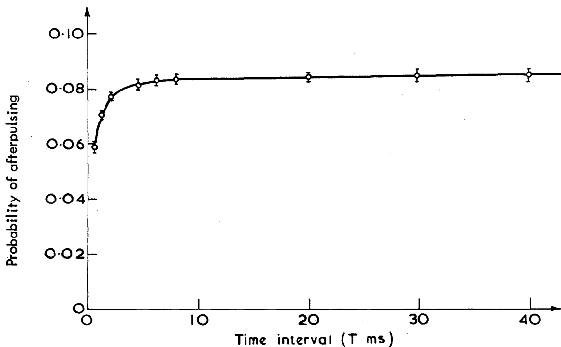
Figure VI-3 - Fractional number of afterpulses per main pulse as a function of correlation counting interval.
