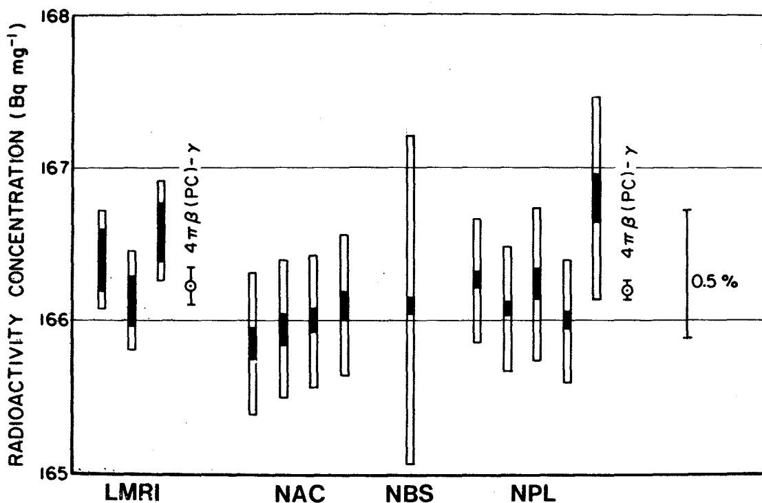
Figure VII-2 - Activities obtained by 4\pi\beta(\text{LS})-\gamma coincidence counting.
