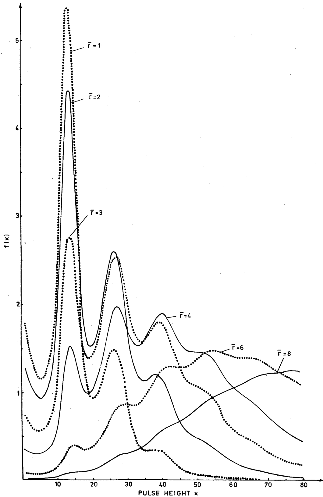
Figure IV-2 - Calculated pulse-height distributions for an input to the first dynode distributed according to Poisson statistics with means of \bar{r} from 1 to 8 (73 Hou) (courtesy North-Holland Publishing Company, Amsterdam).
