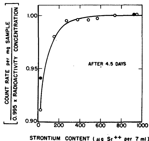
Figure II-3 - Relative loss in count rate due to sample adsorption for ten counting samples containing different amounts of strontium carrier and chelating agent: ○ strontium only, ● strontium + 0.2 mmol HDEHP. Each vial contained \approx 75 ml of aqueous sample in 7 ml of a commercial emulsion scintillator (from measurements made at NBS).
