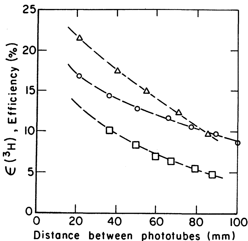
Figure III-4 - ^3\text{H} counting efficiency as a function of separation distance between the phototubes, after Kaufman et al. (60 Kau).
