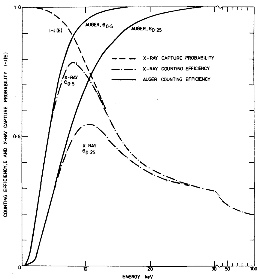
Figure IV-8 - Counting efficiency for X rays and Auger electrons, and X-ray capture probabilities (72 Gib 2) (courtesy Pergamon Press Ltd., Oxford).
