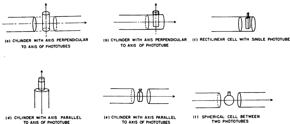
Figure III-3 - Geometrical arrangements of sample containers and phototubes often used in high-efficiency LS systems.
