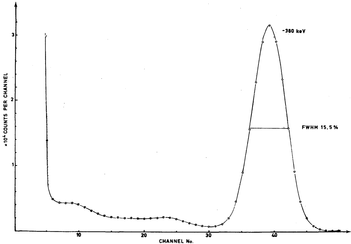
Figure IV-4 - Measured pulse-height distribution of ^{113}\text{Sn} + ^{113}\text{In}^m (73 Hou) (courtesy North-Holland Publishing Company, Amsterdam).
