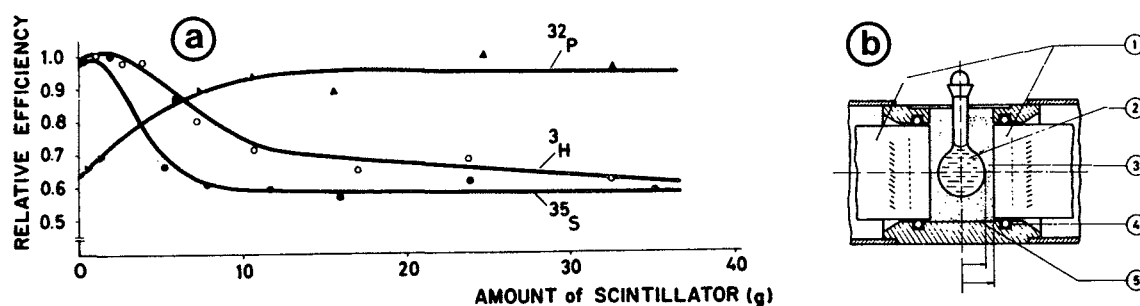
Figure III-5 - (a) Relative counting efficiency as a function of mass of scintillator for system employing spherical vials.
