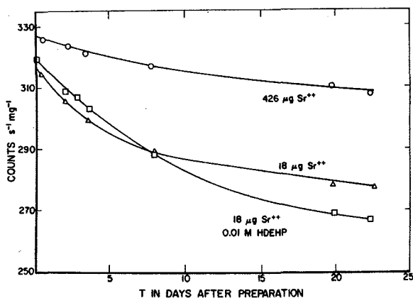
Figure II-2 - Loss in count rate observed for some ^{89}\text{Sr} counting samples prepared using a commercial emulsion scintillator. Measurements were made at 6 °C using a Packard TriCarb, with a window fixed by a single low-level discriminator. The counting efficiency in this window was 0.995. The counting samples consisted of \approx 75 mg of aqueous solution ( \text{SrCl}_2 in an aqueous solution of 0.1 mol HCl per \text{dm}^3 ) in 15 ml of emulsion scintillator in borosilicate-glass vials (from measurements made at NBS).
