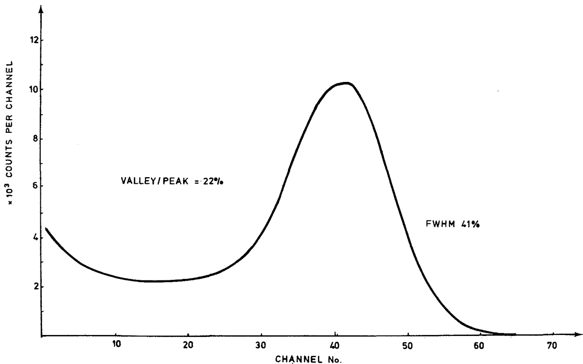
Figure IV-1 - Mono spectrum for an electron-multiplier phototube of type RCA 8850 (73 Hou) (courtesy North-Holland Publishing Company, Amsterdam).
