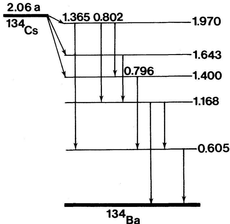
Figure VII-1 - Decay scheme for ^{134}\text{Cs} .
