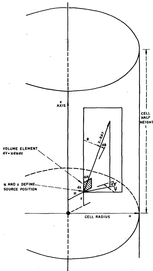
Figure IV-7 - Geometry used in calculating the escape of photon radiation from the scintillator cell (72 Gib 2) (courtesy Pergamon Press Ltd., Oxford).
