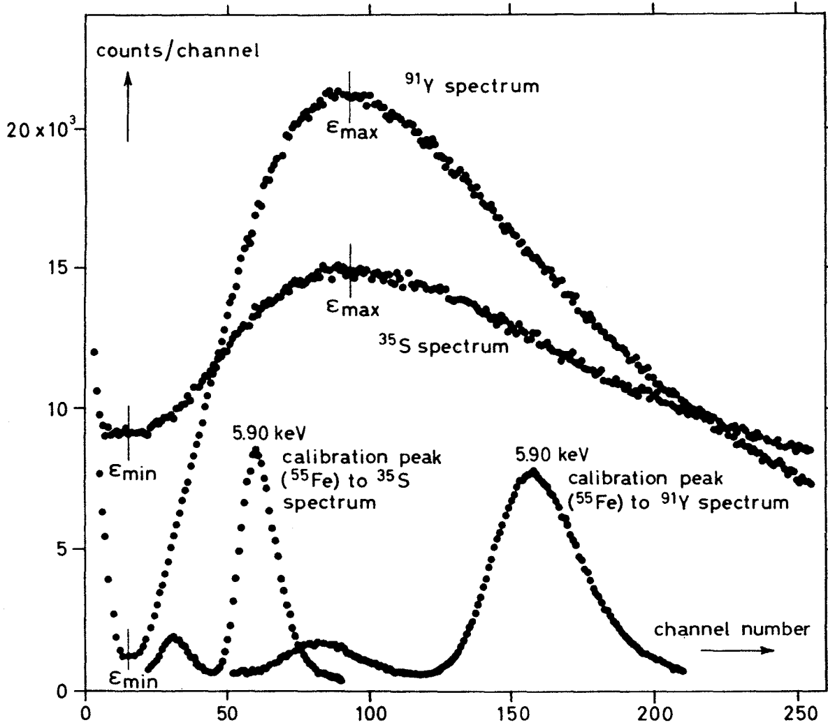
Fig. 1 - Pulse height spectra for ^{91}\text{Y} and ^{35}\text{S} in a 2\pi proportional counter using argon plus 2% methane. (Note: the external amplification was different for the two spectra) (from [3], courtesy IAEA, Vienna).
