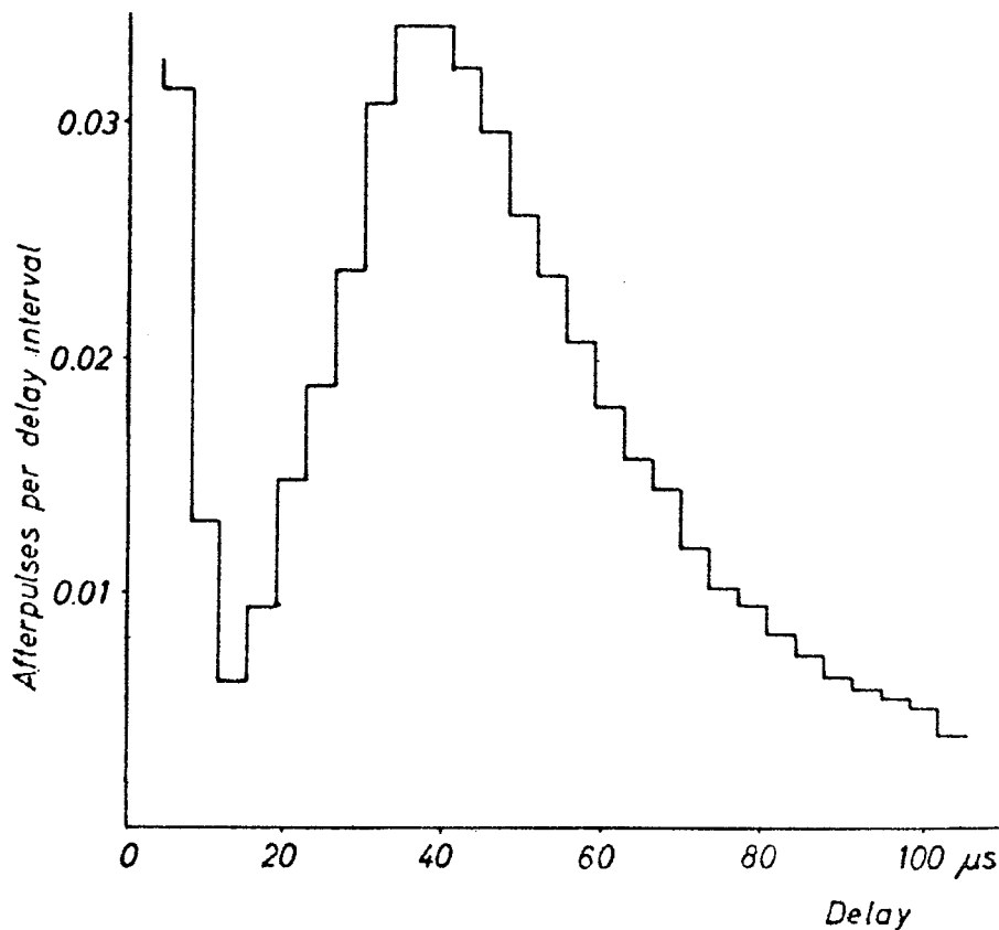
Fig. 9 - Time-interval distribution of spurious pulses for ^{147}\text{Pm} dissolved in a liquid scintillator. Start pulses correspond to an energy loss of 30 to 90 keV (from [21], courtesy North-Holland Publishing Company, Amsterdam).
