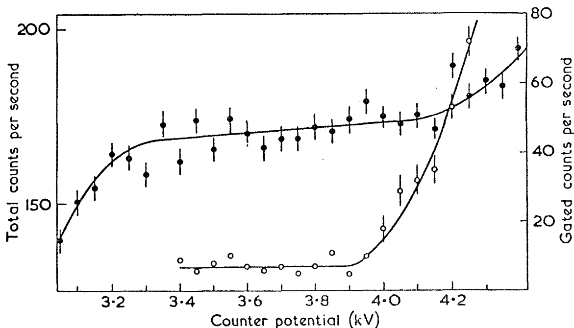
Fig. 4 - A plateau plot (solid circles, left-hand ordinate) and the gated counts as described in the text (open circles, right-hand ordinate) (from [13], courtesy Institute of Physics, London).
