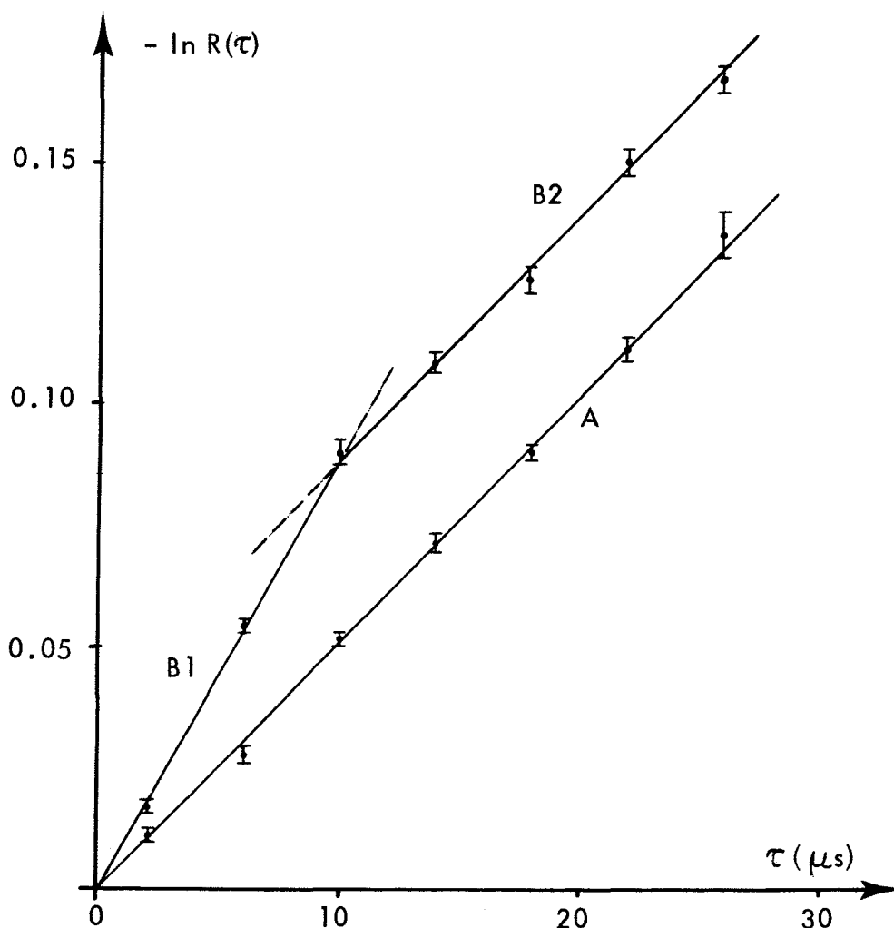
Fig. 5 - Measurement of the correlation function R(\tau) , for the approximate parameters N_{\text{sing}} = 2\,500\text{ s}^{-1} , N_{\text{pair}} = 0 or 900\text{ s}^{-1} and \lambda^{-1} \equiv \tau_0 = 10\text{ }\mu\text{s} . The theoretical curves given for comparison are
