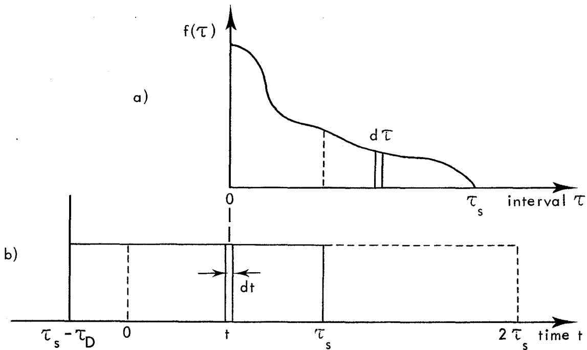
Fig. 10 - a) A hypothetical interval density f(\tau) of spurious pulses as a function of time interval \tau .
