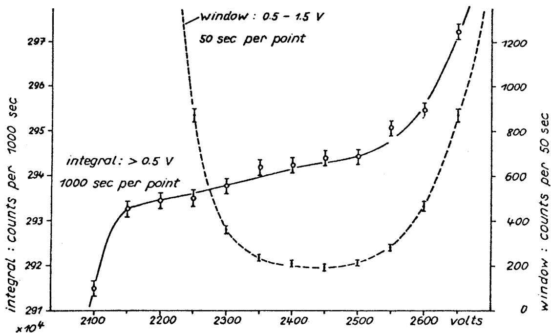
Fig. 2 - A plateau plot (left-hand ordinate) together with the output from a single-channel analyser with a fixed window (right-hand ordinate) for a ^{60}\text{Co} source in a methane filled proportional counter (from [4], courtesy IAEA, Vienna).
