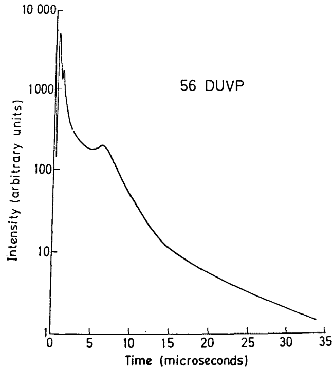
Fig. 7 - Time-interval distribution of spurious pulses in a phototube type 56 DUVP (from [12]).
