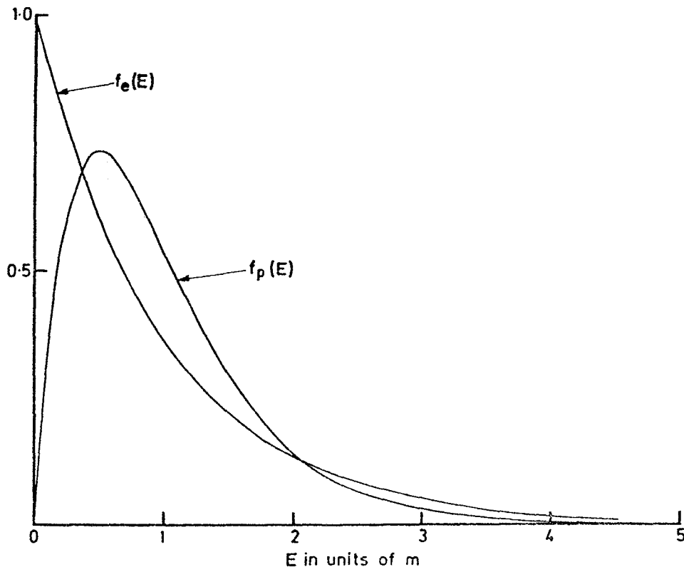
Fig. 6 - Theoretical single-electron pulse-height distributions. The mean of both distributions is m .
