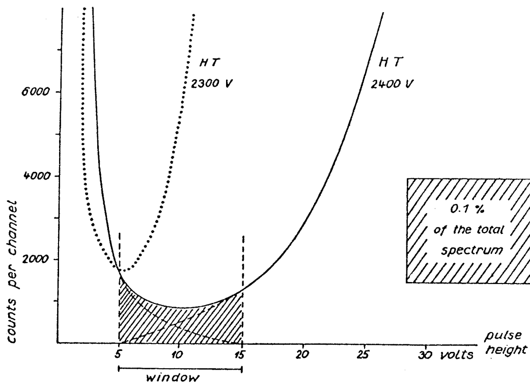
Fig. 3 - First part of the pulse-height spectrum of a ^{137}\text{Cs} source in a 4\pi proportional counter (from [4], courtesy IAEA, Vienna).
