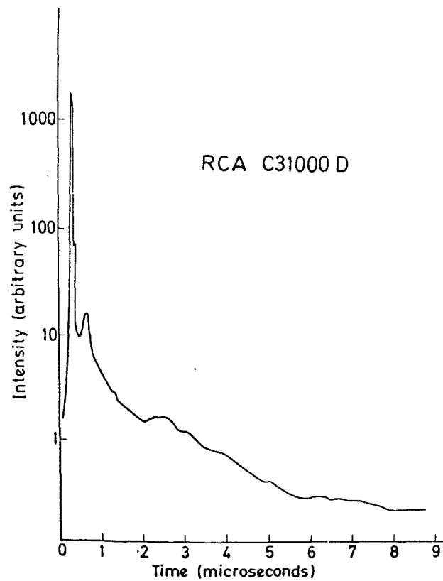
Fig. 8 - Time-interval distribution of spurious pulses in a phototube type RCA C31000 D (from [2], courtesy North-Holland Publishing Company, Amsterdam).
