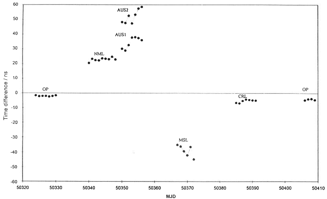
Figure 2. Daily averages of dt_{k,i} for each laboratory.
