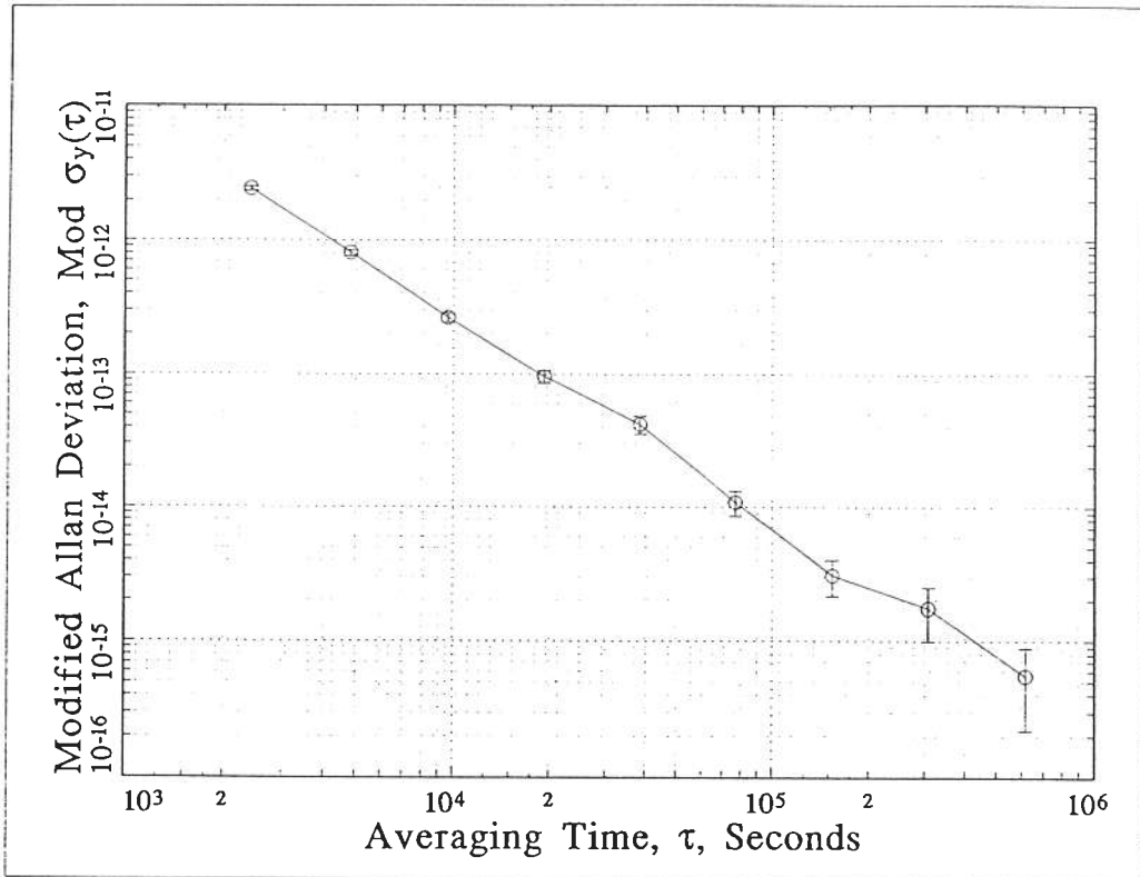
Figure 1. Square root of the modified Allan variance of the time series dt_{OP} for the period 3 - 18 July 1996.
