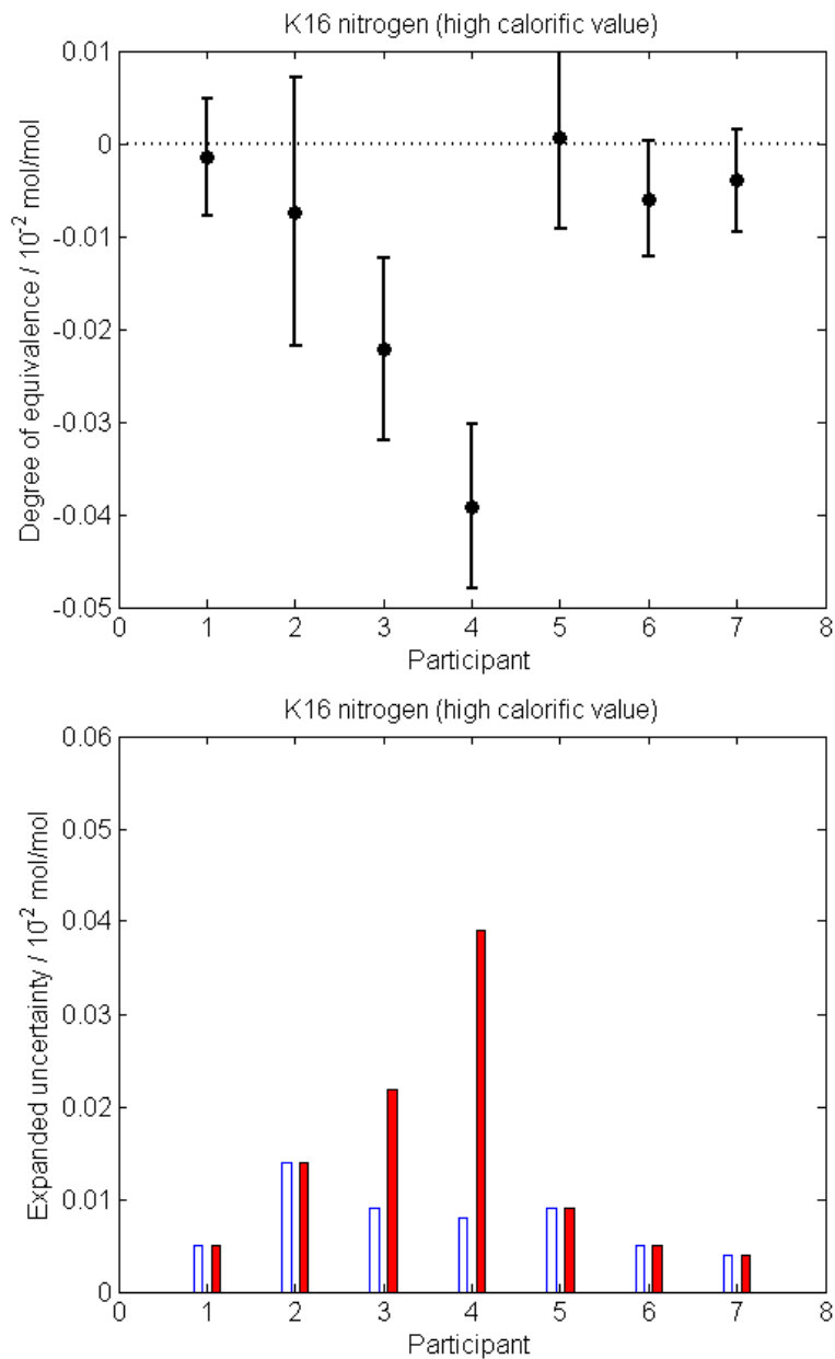
Figure 1: DoEs depicted as ‘error bars’ [d_i - U(d_i), d_i + U(d_i)] for the participants (top), and expanded uncertainties U(x_i) and proposed U(\text{cmc}_i) (bottom) for the species nitrogen (high calorific value) in CCQM-K16.
