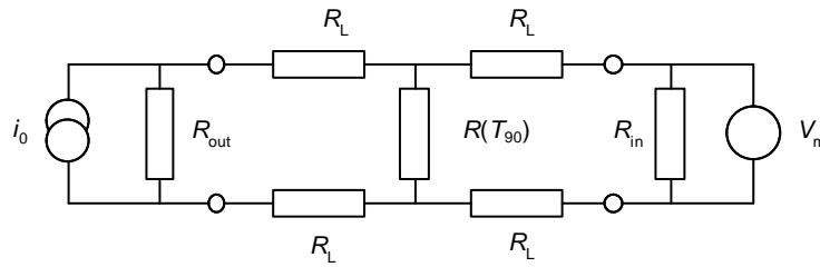
Figure 4. The equivalent circuit for a 4-terminal resistance measurement.
