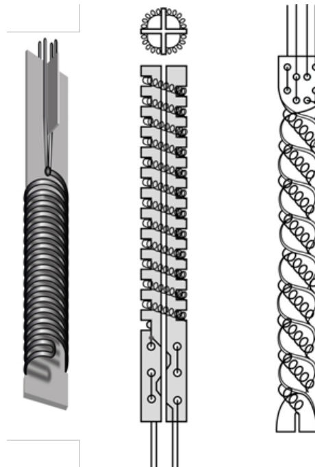
Figure 3. Schematic designs of sensitive elements of SPRTs: HTSPRT with a simple bifilar platinum coil supported on a notched high-purity silica plate, R(0.01\text{ °C}) \sim 0.25\ \Omega (left); LSPRT with the platinum coil laid in notches in a silica cross, R(0.01\text{ °C}) \sim 25\ \Omega (centre and top-view); LSPRT with the platinum coil laid in the helical turns of a twisted silica plate, R(0.01\text{ °C}) \sim 25\ \Omega (right). In all cases two platinum wires are welded to the coils at each end to create four-lead connections (“Y” joints). (Illustration published on courtesy from FLUKE®)
