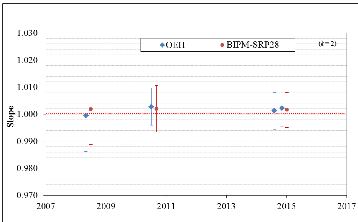
Figure 2 : Results of the comparisons between SRP27, SRP28 and OEH SRP21 performed at the BIPM during the course of the key comparison BIPM.QM-K1. Uncertainties are calculated at k=2 , with the uncertainty budget in use at the time of each comparison.
